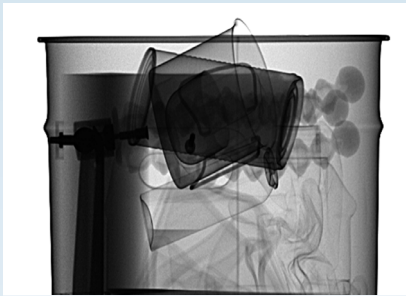
Identification of neutron absorber in waste
